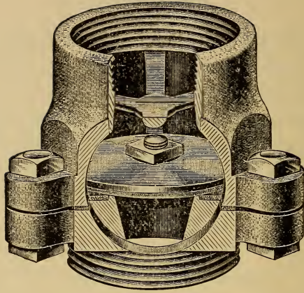
FIG. 11.—CHECK VALVE.
